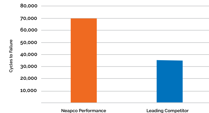
High Cycle/Low Torque Fatigue Comparison
