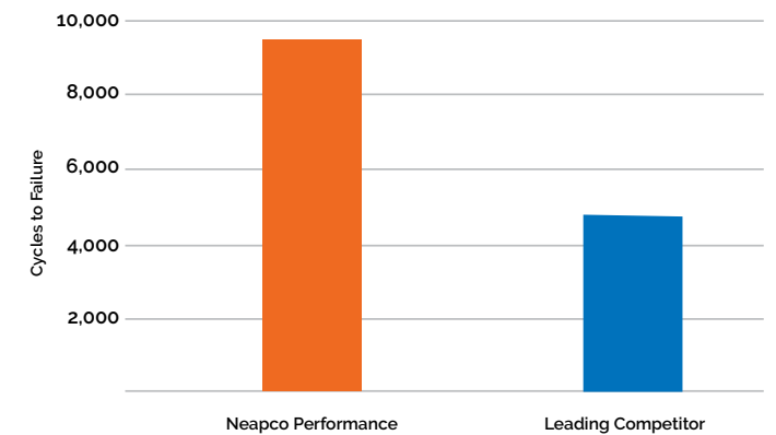
Low Cycle/High Torque Fatigue Comparison
